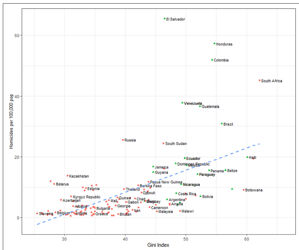
Figure 3 Homicides and Inequality, World.
